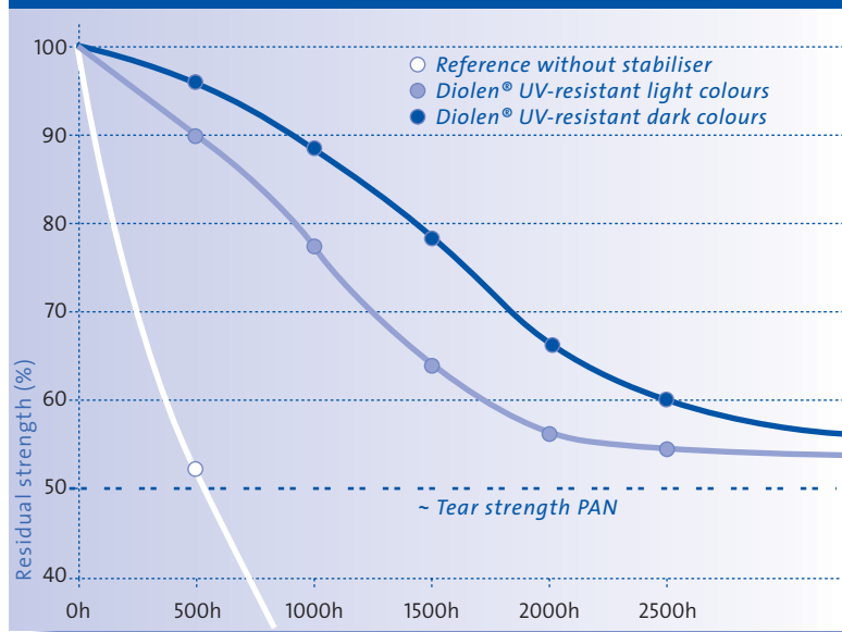
Diolen® UV-resistant in comparison with standard PES Mechanical test (weathered according to DIN EN 105 B04)
